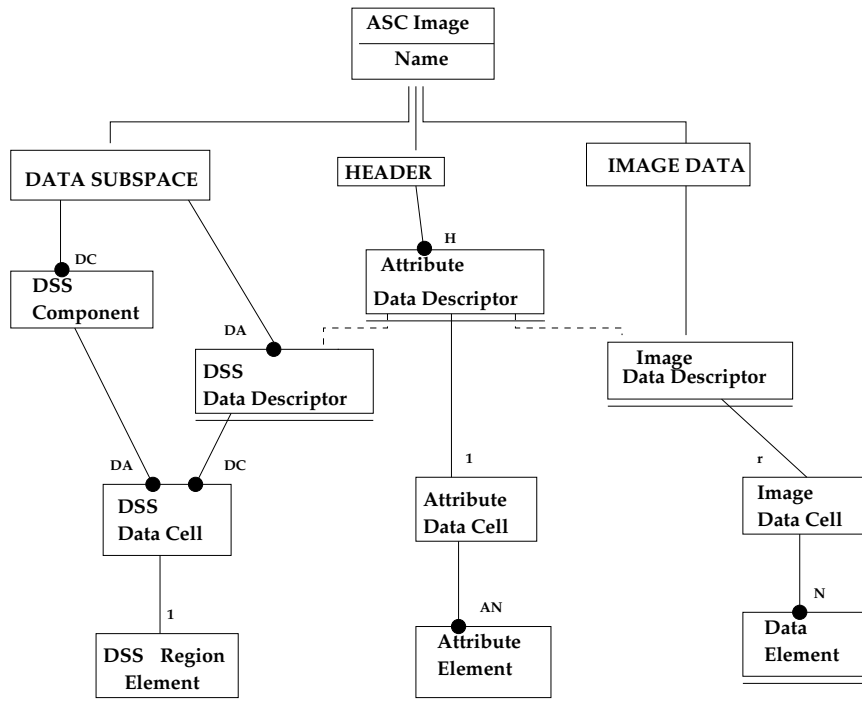
Figure 11: Data Model 7: ASC Image Model, identical to Table Model but without Table Row and with only one Column Descriptor (Image Descriptor).
