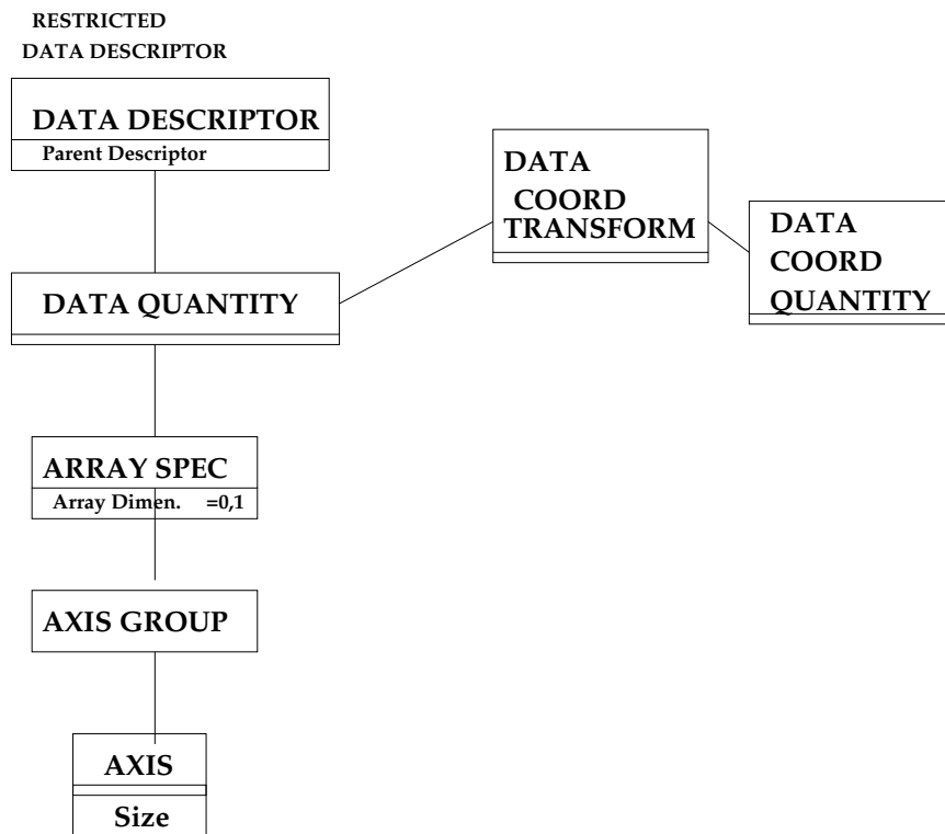
Figure 10: Data Model 6: Restricted Data Descriptor, used in Attribute Data Descriptor and DSS Data Descriptor. Does not support full Array/Image functionality.
