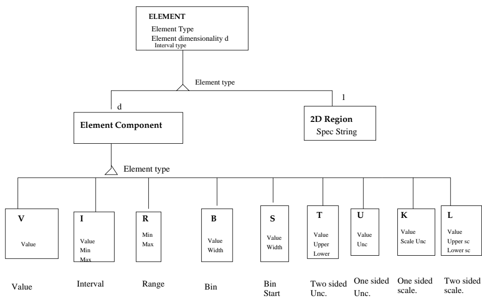
Figure 8: Data Model 5: The Element object, used to store the actual values. There may be many elements described by a single Quantity. There is one Element component for each dimension of the element, except if systematic uncertainties are included in which case there may be up to three Element components for each dimension.
