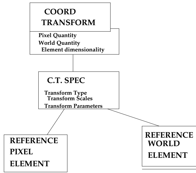
Figure 6: Data Model 3: Use of the Coordinate Transform. The Coordinate Transform object includes the reference pixel element and the reference world element, as well as the world Quantity. The World element is then defined in terms of the Pixel element and quantity with which the Transform is associated.
