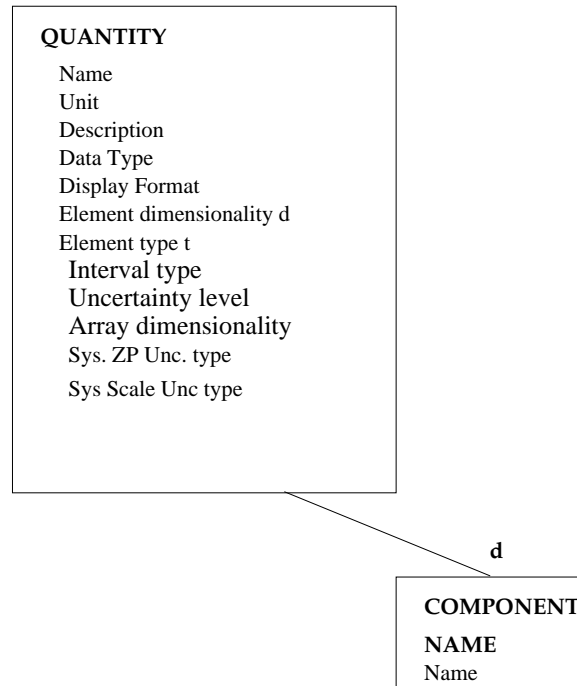
Figure 5: Data Model 2: The Quantity object, used to describe the structure and properties of named quantities (header attributes, table columns, data subspace axes, world coordinates
