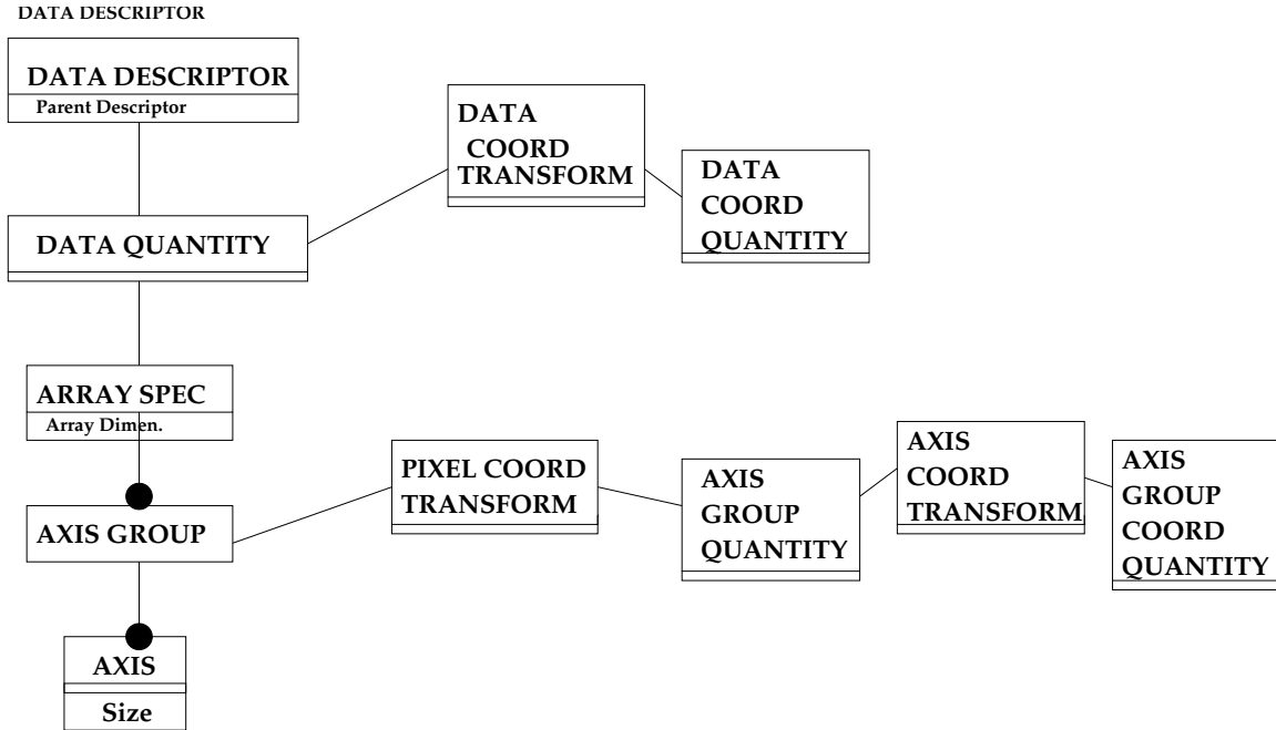
Figure 7: Data Model 4: The Data Descriptor object, which consists of a named Quantity and Array Specification with which data cells will be associated, as well as implicitly defined associated Quantities which label the axes and provide coordinate systems.
